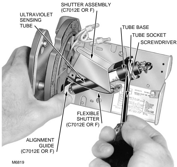
Fig. 20. Replacing ultraviolet radiation sensing tube.
