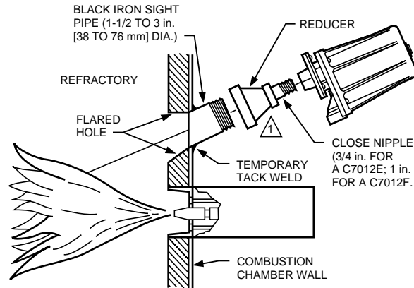
Fig. 5. Typical mounting of C7012.
