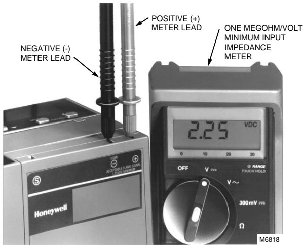
Fig. 19. Measuring voltage flame signal with 7800 SERIES controls.
