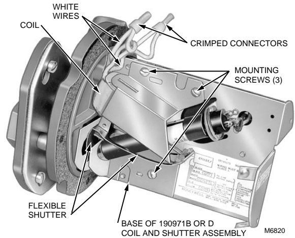
Fig. 21. Replacing coil and shutter assembly on C7012E,F.
