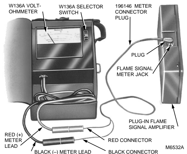
Fig. 17. Measuring microamp flame signal.
