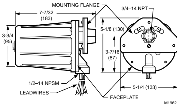
Fig. 1. Dimensions of C7012A,E, and G in in. (mm).
